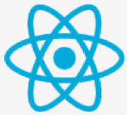
React Native
